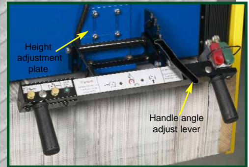
Standard Handle
