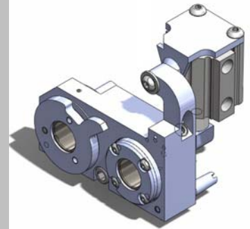
AS-109106-000 LOWER DRIVE CARTRIDGE,LH
